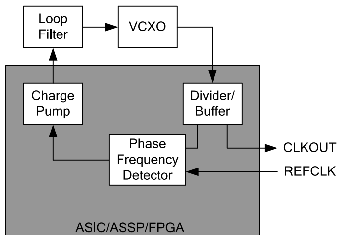
Figure 3. Partially Integrated PLL in ASIC
