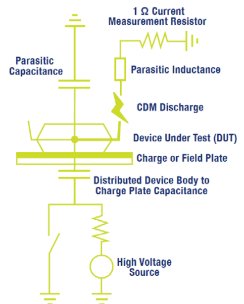
Figure 5 – Typical test setup for capacitive discharge model EST testing.
