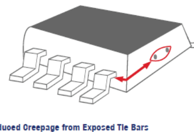
Figure 3 – Exposed tie bars (circled) reduce the amount of creepage.
