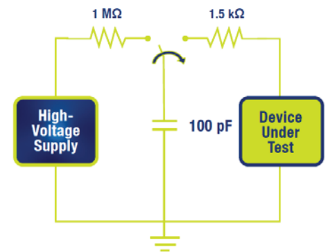
Figure 4 – Typical test setup for human body model ESD testing.
