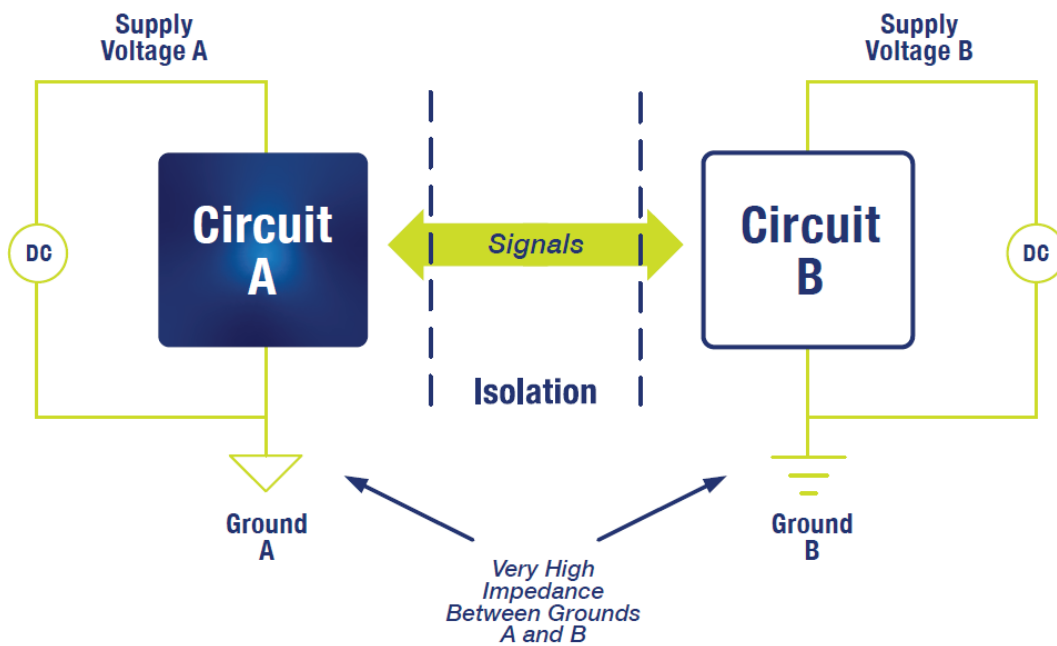
Figure 1 – Isolation creates a very high impedance between two grounds in a system, effectively eliminating the electrical connection between them.
