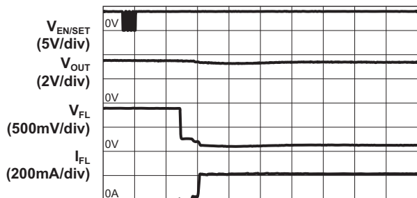
Movie Mode Turn On Characteristic
