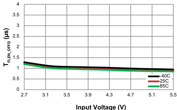
Flash Mode Turn Off Time vs Input Voltage ( I_{FL} = 1.5\text{A} ; C_{OUT} = 2.2\mu\text{F} ; L = 1\mu\text{H} )
