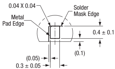
Detail D Pad Scale: 2X X This rotation X Rotated 180°
