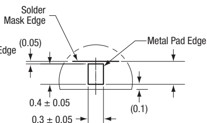
Detail B Pad Scale: 2X X This rotation X Rotated 180° X Rotated 90° CW
