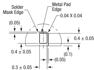
Detail C Pad Scale: 2X 1X This rotation 1X Rotated 180° 1X Rotated 90° CCW 1X Mirrored 45°
