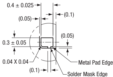
Detail E Pad Scale: 2X X This rotation X Mirrored 180°
