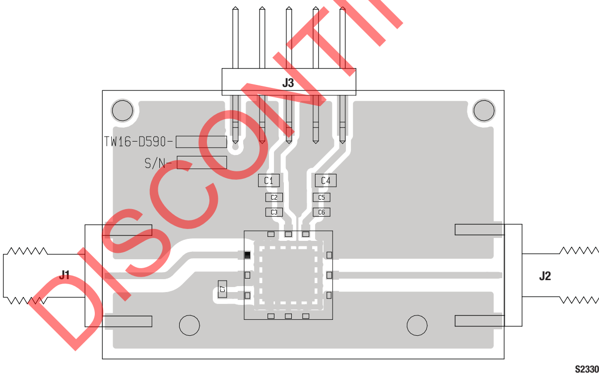
Figure 21. SKY65187-11 Evaluation Board Assembly Drawing
