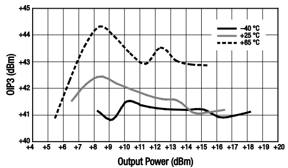
Figure 14. OIP3 vs Output Power Over Temperature
