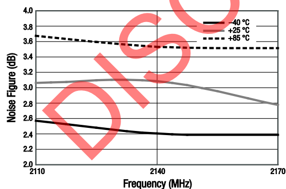
Figure 19. Noise Figure vs Frequency Over Temperature
