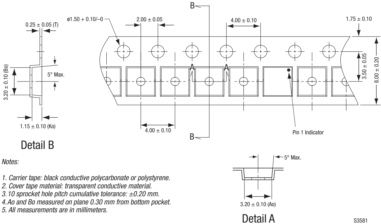
Figure 10. SKY66008-11 Tape and Reel Dimensions
