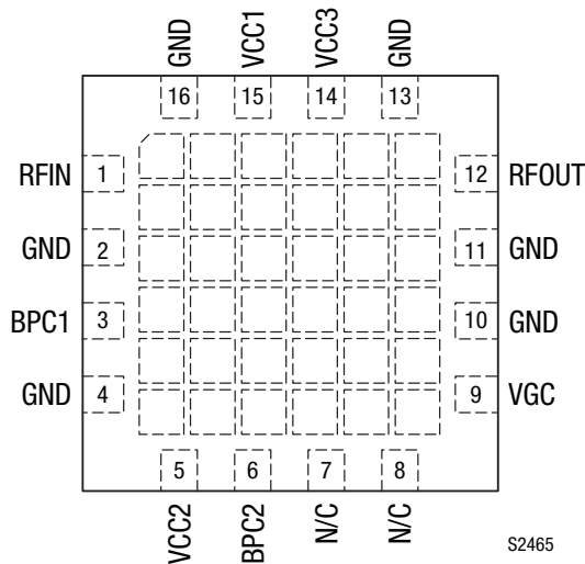
Figure 2. SKY65375-11 Pinout (Top View)
