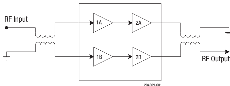
Figure 1. ACA2429 Block Diagram
