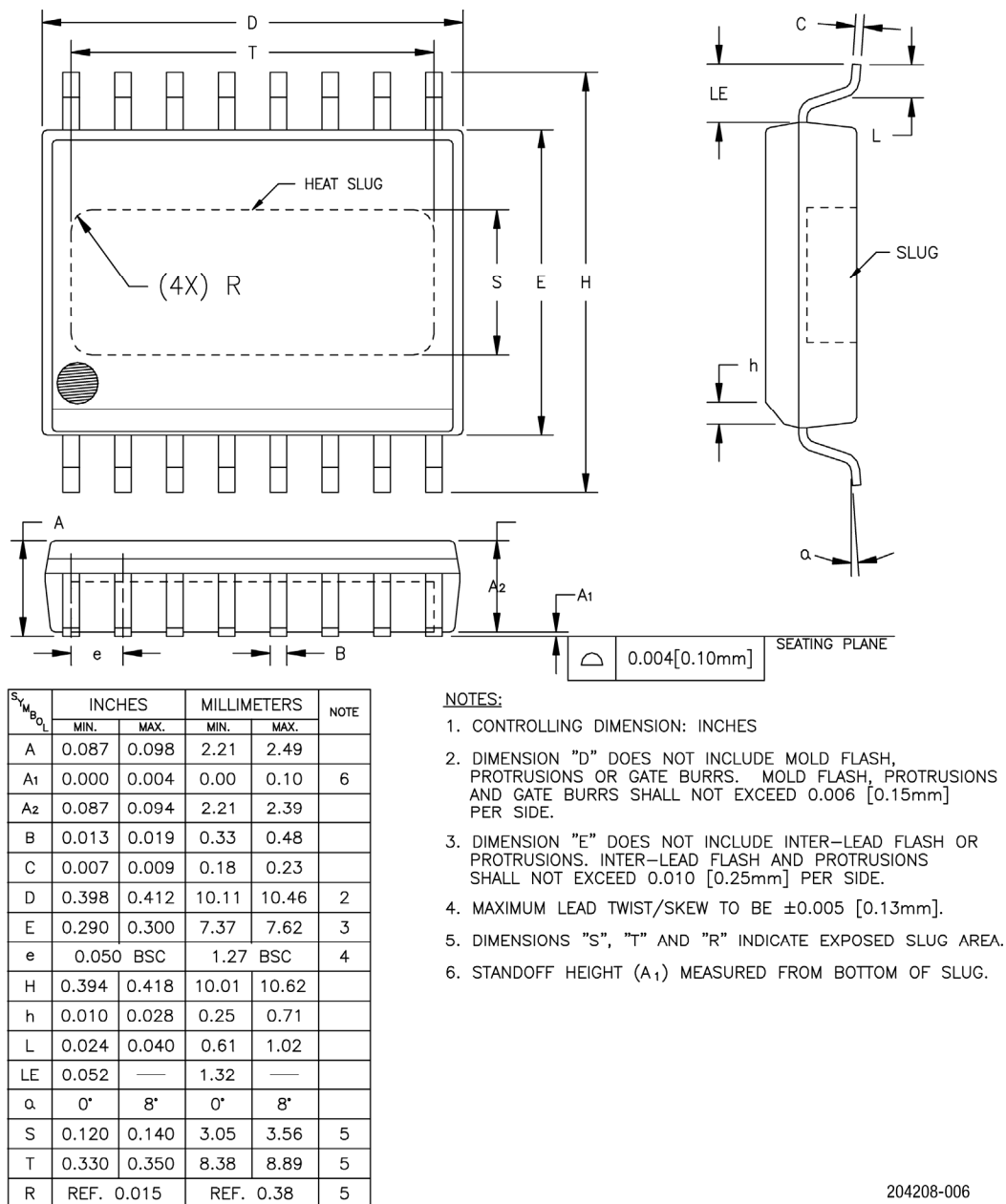
Figure 6. ACA2429 Package Dimensions
