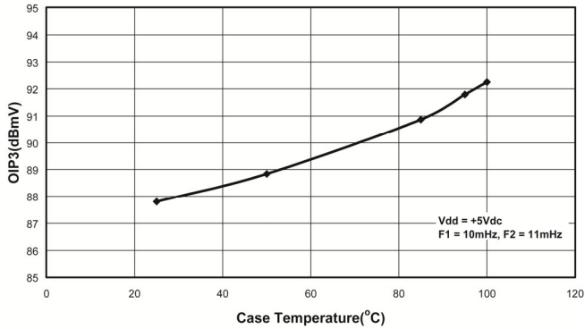
Figure 9. Output Third Order Intercept Point (OIP3) vs Temperature (V DD = +5 V, f 1 = 10 MHz, f 2 = 11 MHz)
