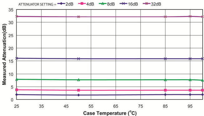
Figure 12. Attenuator Accuracy over Temperature (V DD = +5 V, f 1 = 10 MHz)
