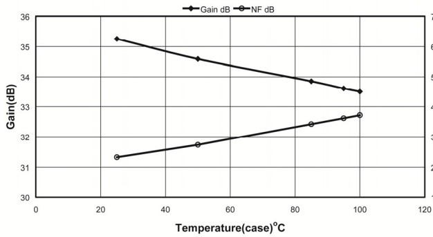
Figure 5. Gain and Noise Figure vs Temperature (VDD = +5 Vdc, f1 = 10 MHz)
