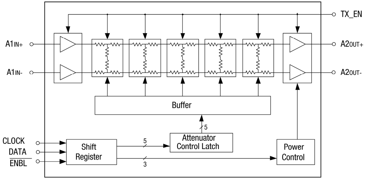
Figure 1. ARA2017 Functional Block Diagram
