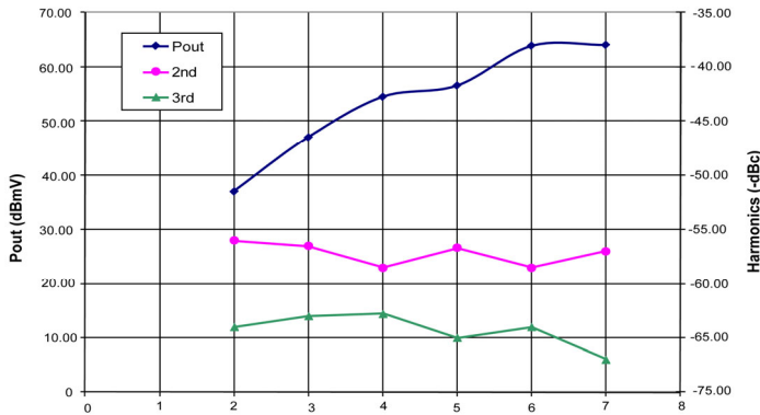
Figure 14. P out and Harmonics vs Power Control Setting
