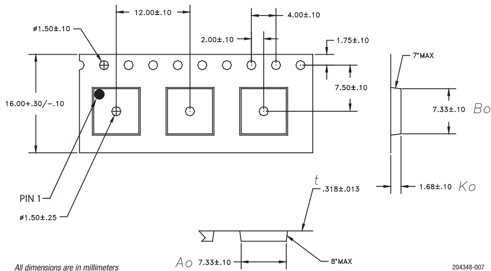
Figure 7. AWB7239 Tape and Reel Dimensions
