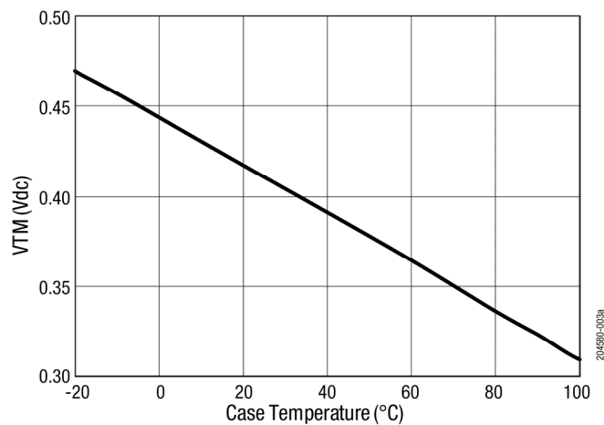
Figure 3. VTM vs Case Temperature
