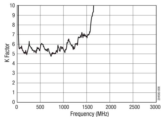
Figure 9. K vs Frequency ( T_{CASE} = +85\text{ }^{\circ}\text{C} ) Gain Control= 12 Vdc
