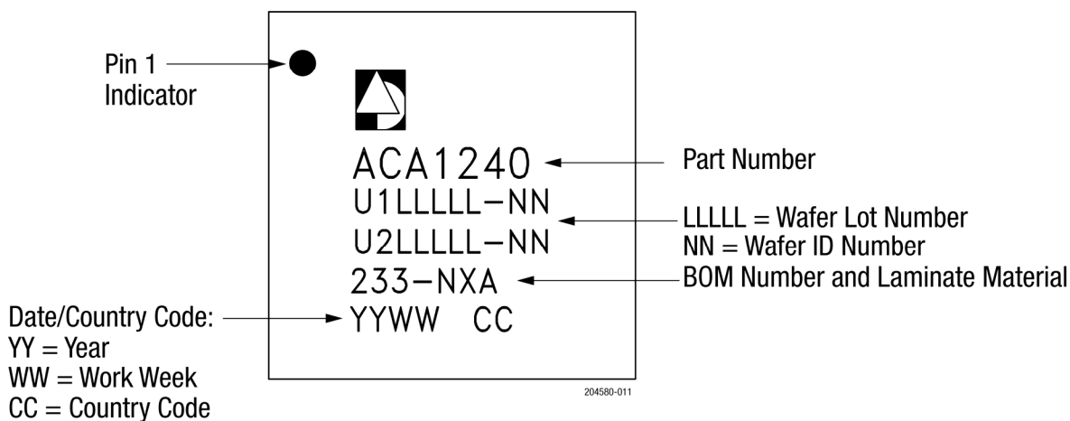
Figure 12. Typical Part Marking
