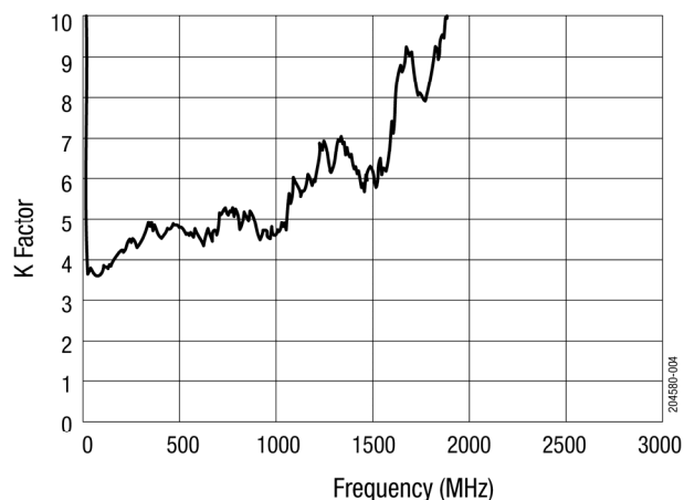
Figure 5. K vs Frequency ( T_{CASE} = -20\text{ }^{\circ}\text{C} ) Gain Control= 12 Vdc
