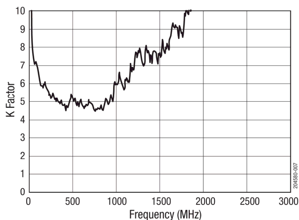
Figure 8. K vs Frequency ( T_{CASE} = +45\text{ }^{\circ}\text{C} ) Gain Control= 12 Vdc
