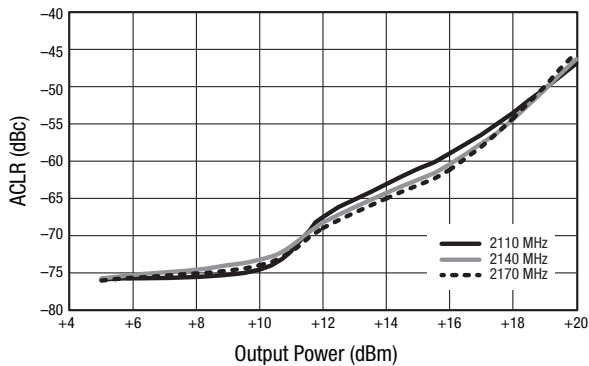
Figure 7. ACLR vs Output Power (WCDMA Test Model 1 w/64 DPCH)
