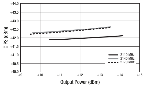
Figure 8. OIP3 vs Output Power (Δf = 1 MHz)
