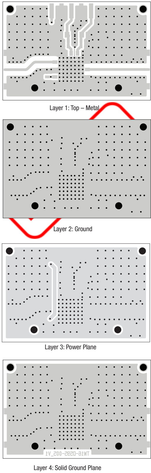
Figure 12. SKY65387-11 Evaluation Board Layer Detail
