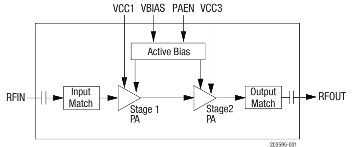
Figure 1. SKY66295-21 Block Diagram
