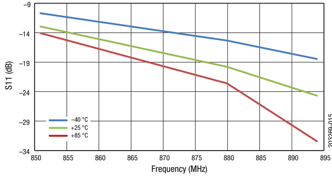
Figure 15. Input Return Loss vs Frequency Across Temperature (Small Signal, PIN = -30 dBm)
