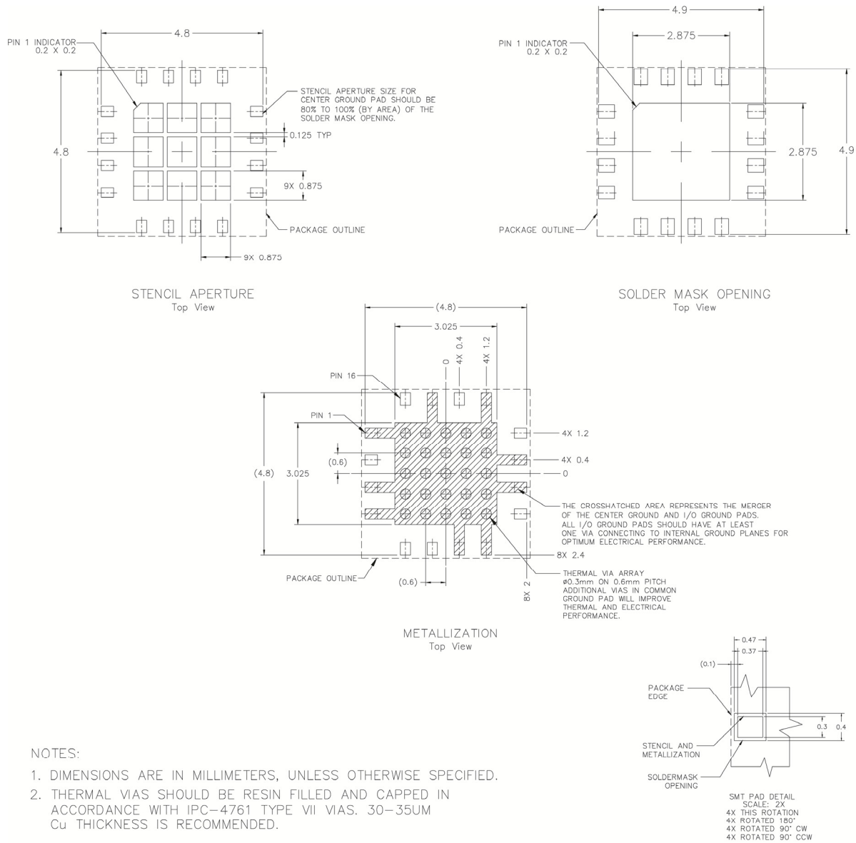
Figure 22. SKY66295-21 PCB Layout Footprint
