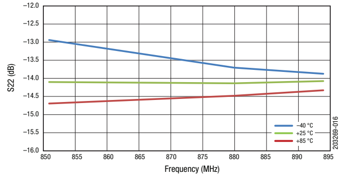
Figure 16. Output Return Loss vs Frequency Across Temperature (Small Signal, PIN = -30 dBm)
