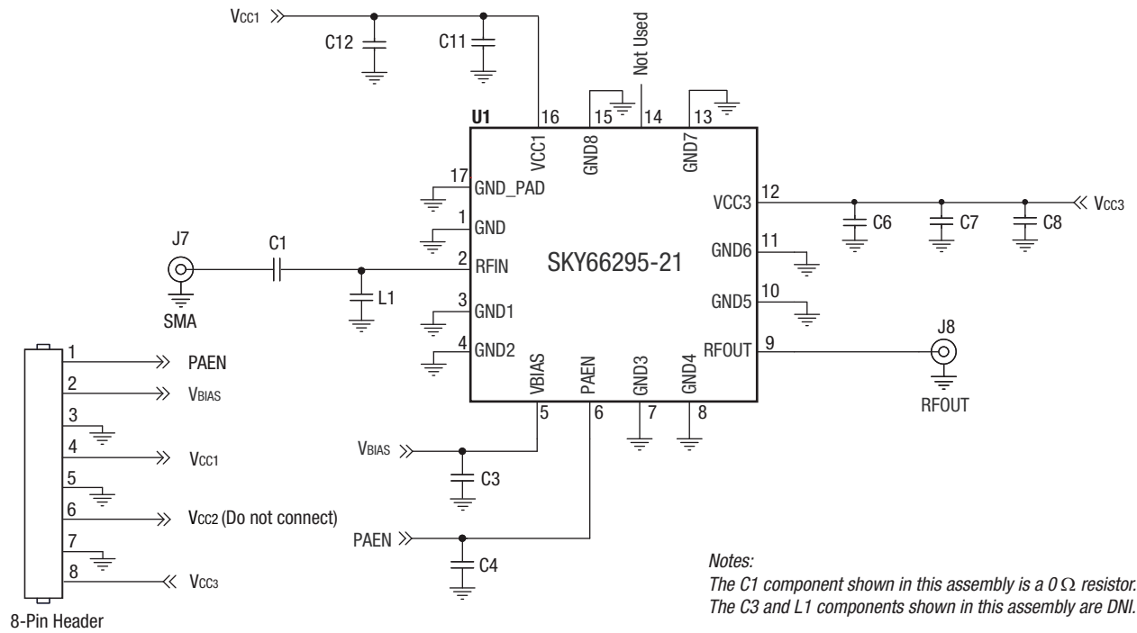
Figure 17. SKY66295-21 Evaluation Board Schematic
