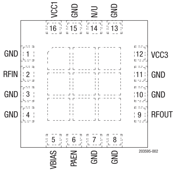
Figure 2. SKY66295-21 Pinout (Top View)
