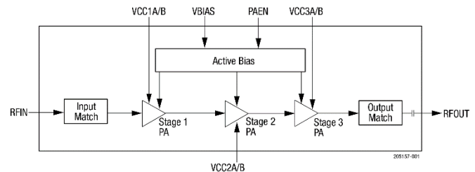
Figure 1. SKY66398-11 Block Diagram
