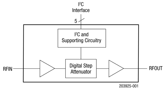
Figure 1. SKY67302-11 Block Diagram
