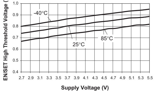
EN/SET High Threshold Voltage vs. Supply Voltage and Temperature
