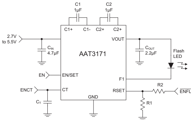
Figure 3: Flash/Torch Control Using the RSET Pin.
