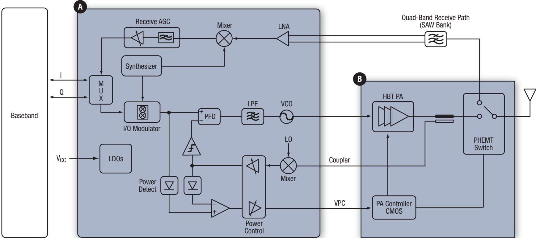
RF Transceiver A SKY74138
