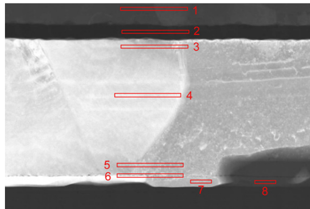
Figure 2 STEM image of Cu Metal 1 on Ohmic
