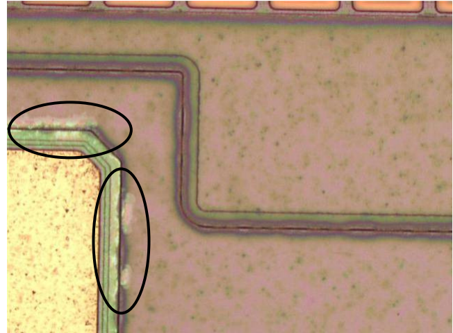
Figure 1 Exposed Cu attacked in pre-clean solution.
