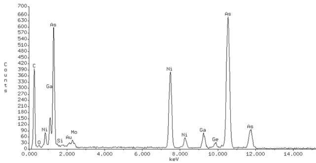
Figure 3 EDX survey of Site 8.
