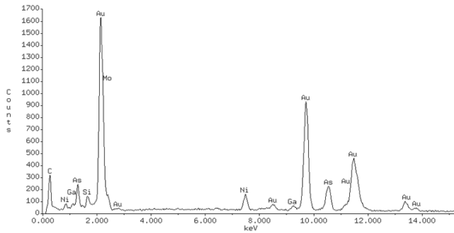
Figure 4 EDX survey of Site 6.
