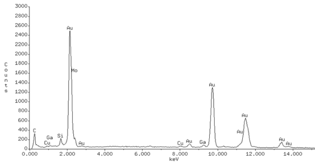
Figure 5 EDX survey of Site 4. Small Cu signal is from the grid.
