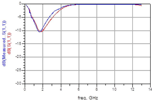
Figure 3. Measured Data (Blue) vs. Modeled Data (Red) for Input Return Loss
