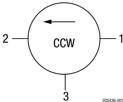
Figure 1. SKYFR-001710 Block Diagram
