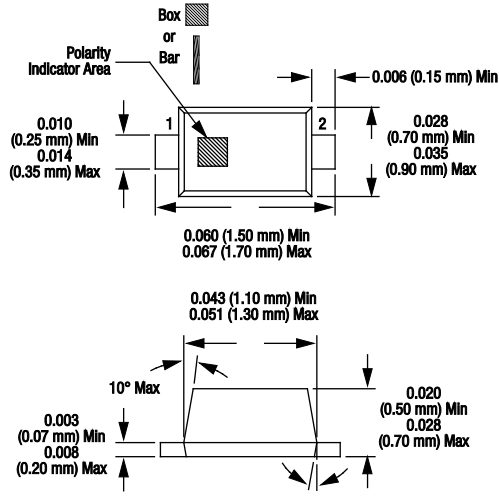
Figure 7. SC-79 Package Dimension Drawing
