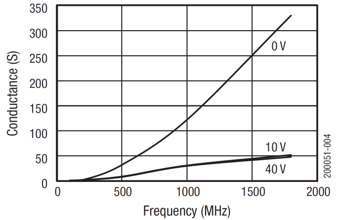
Figure 4. Conductance vs Frequency and Reverse Voltage
