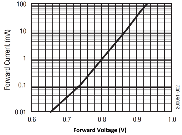
Figure 2. Forward Current vs Voltage
