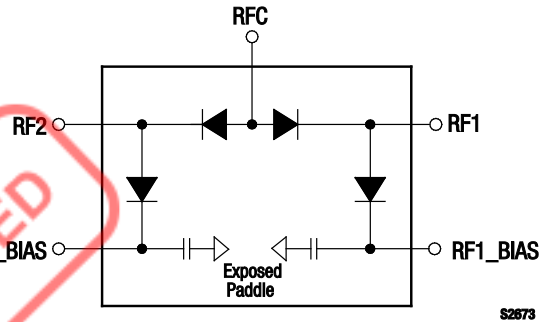
Figure 1. SKY12209-478LF Block Diagram
