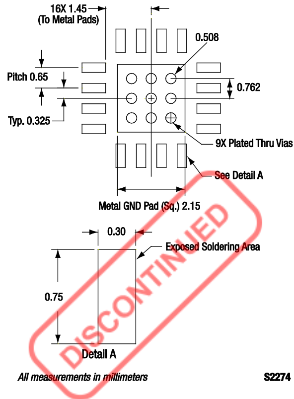
Figure 17. SKY12209-478LF PCB Layout Footprint
