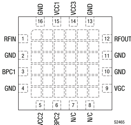
Figure 2. SKY65371-11 Pinout (Top View)
