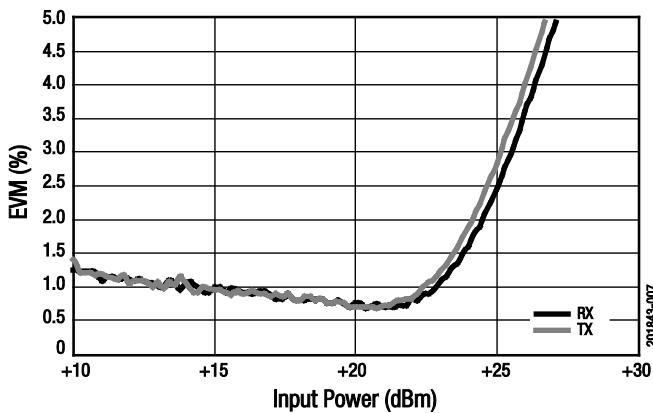
Figure 7. EVM vs Input Power (@ 5.5 GHz, 54 bps)
