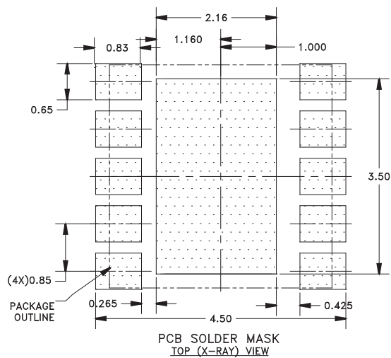
Figure 4: PCB Footprint
