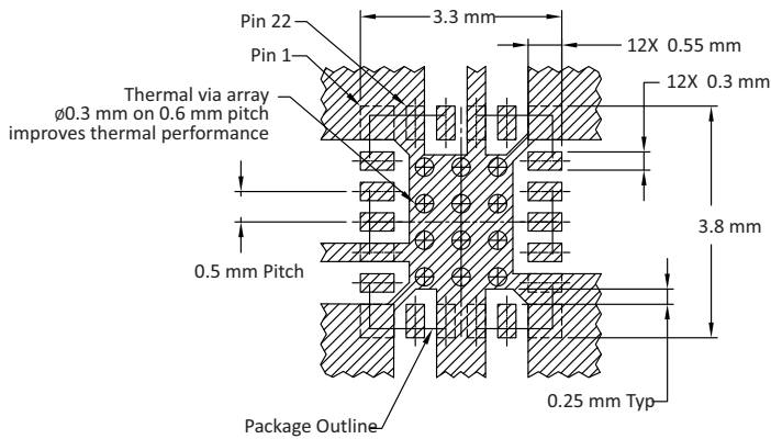
Metallization (Top View)
