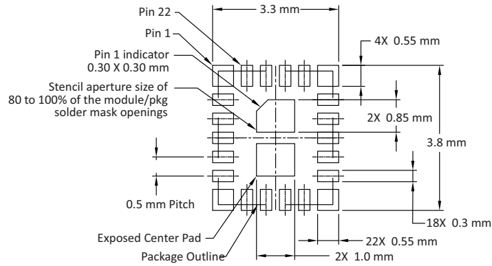
Stencils Aperture (Top View)
