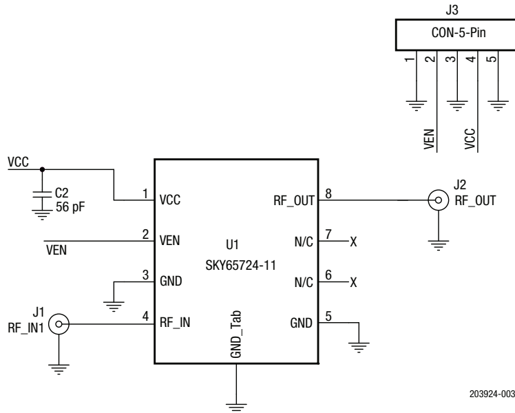
Figure 3. SKY65724-11 Application Schematic
