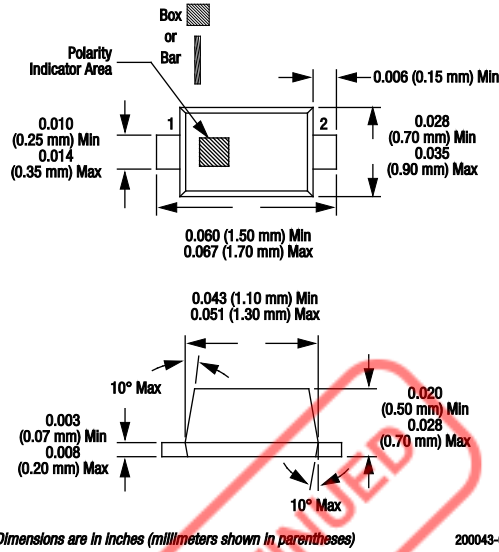
Figure 5. SC-79 Package Dimension Drawing
