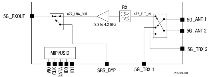
Figure 1. SKY53728-21 Block Diagram
