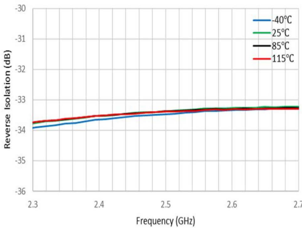
Figure 35. Reverse Isolation vs. Frequency
