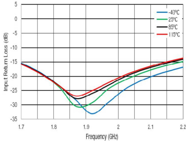
Figure 47. Input Return Loss vs. Frequency
