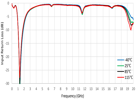
Figure 69. Input Return Loss vs. Frequency
