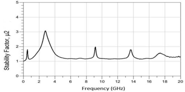
Figure 44. Stability Factor, \mu_2 vs. Frequency at -40\text{ }^\circ\text{C}
