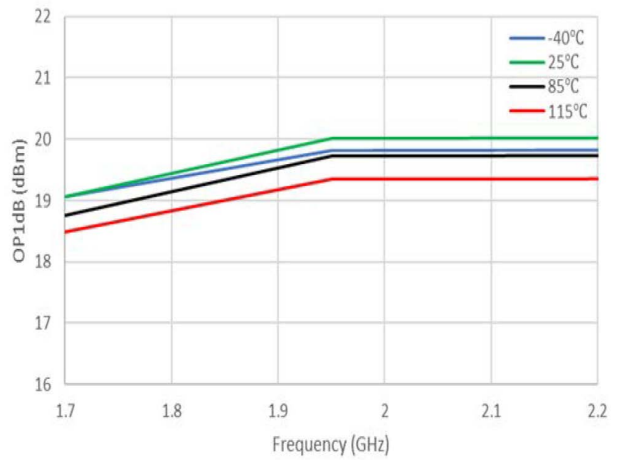
Figure 52. OP1dB vs. Frequency
