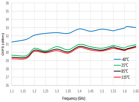
Figure 65. OIP3 vs. Frequency
