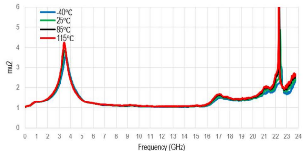
Figure 30. Stability Factor \mu_2 vs. Frequency
