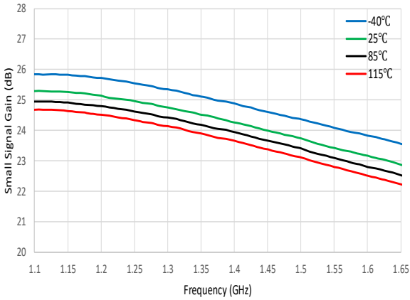
Figure 59. Small Signal Gain vs. Frequency
