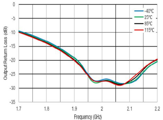
Figure 48. Output Return Loss vs. Frequency
