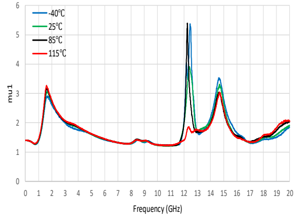
Figure 72. Stability Factor, \mu_1 vs. Frequency
