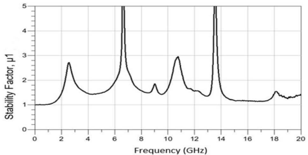
Figure 43. Stability Factor, \mu_1 vs. Frequency at -40\text{ }^\circ\text{C}
