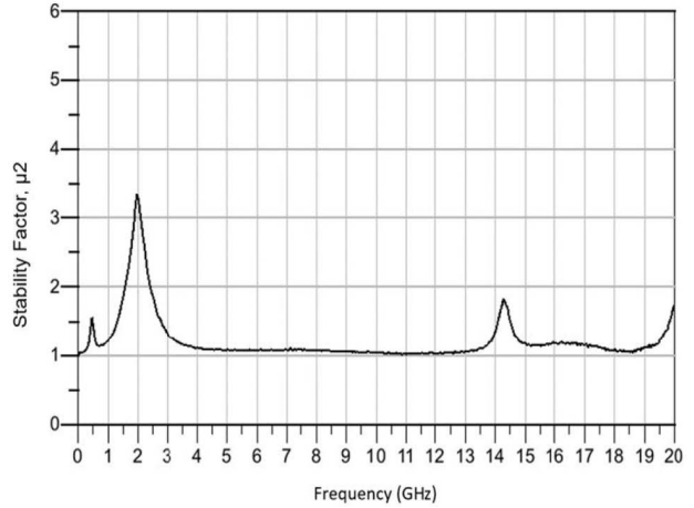
Figure 58. Stability Factor, \mu_2 vs. Frequency at -40\text{ }^\circ\text{C}
