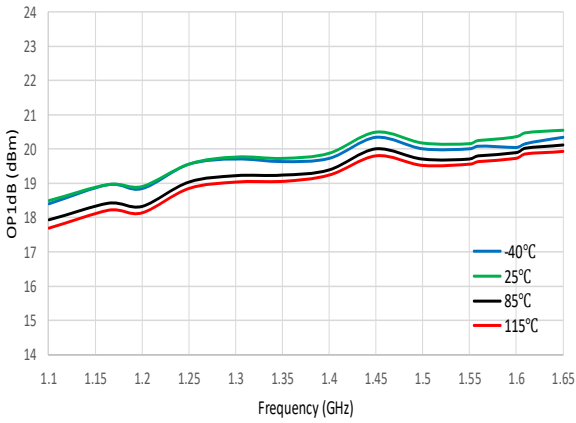
Figure 67. OP1dB vs. Frequency
