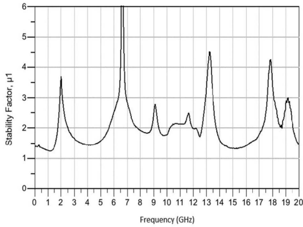
Figure 57. Stability Factor, \mu_1 vs. Frequency at -40\text{ }^\circ\text{C}
