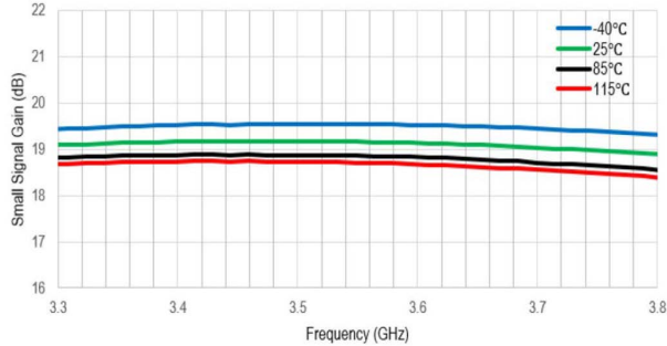
Figure 17. Small Signal Gain vs. Frequency
