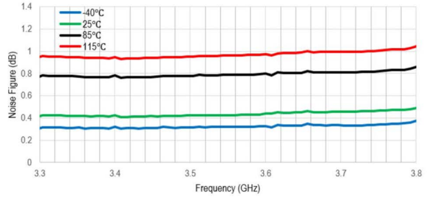
Figure 18. Noise Figure vs. Frequency
