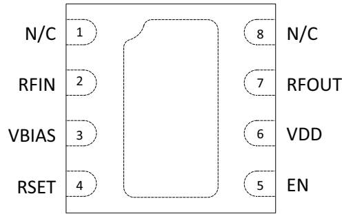
Figure 2. Pinout (Top View)
