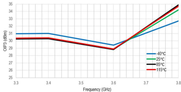
Figure 23. OIP3 vs. Frequency
