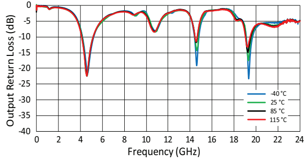
Figure 14. Output Return Loss vs. Frequency
