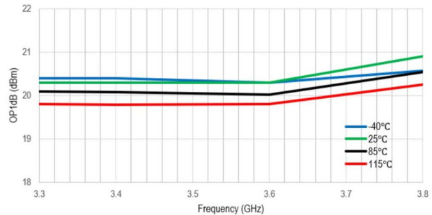
Figure 24. OP1dB vs. Frequency
