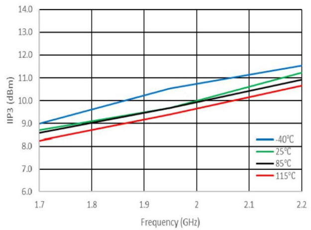
Figure 50. IIP3 vs. Frequency
