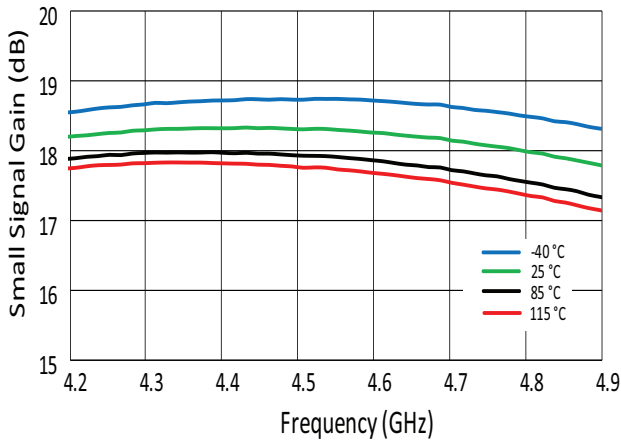
Figure 3. Small Signal Gain vs. Frequency
