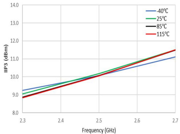
Figure 36. IIP3 vs. Frequency
