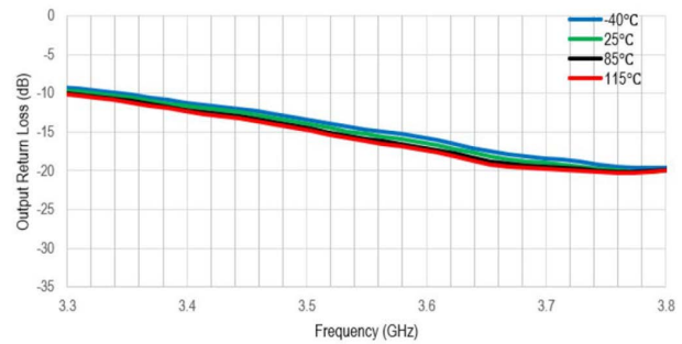
Figure 20. Output Return Loss vs. Frequency
