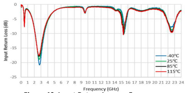
Figure 40. Input Return Loss vs. Frequency
