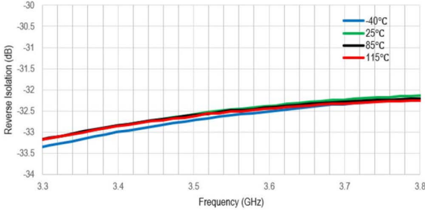
Figure 21. Reverse Isolation vs. Frequency
