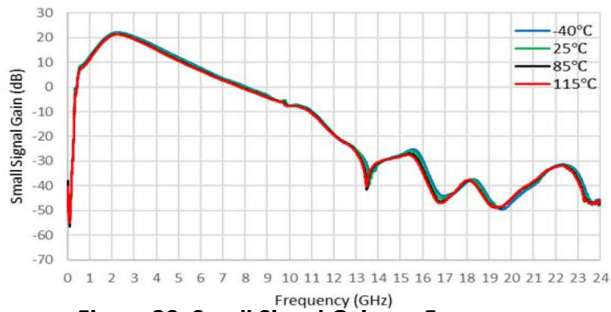
Figure 39. Small Signal Gain vs. Frequency
