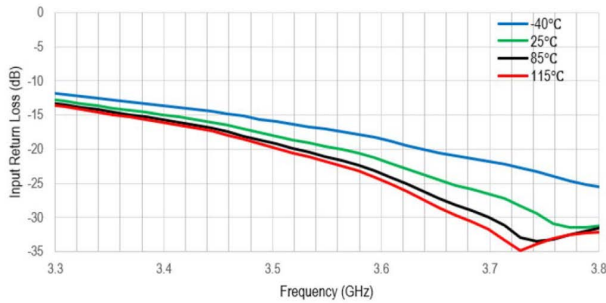
Figure 19. Input Return Loss vs. Frequency
