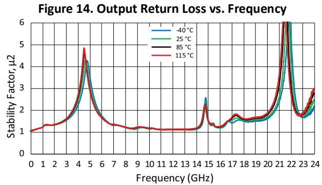
Figure 16. Stability Factor, \mu_2 vs. Frequency
