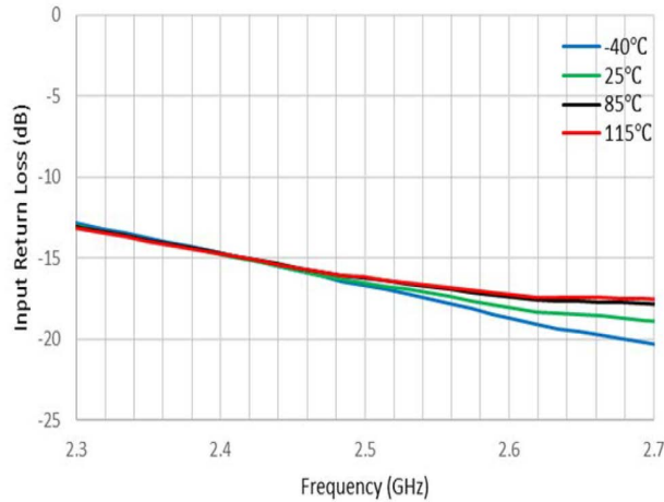
Figure 33. Input Return Loss vs. Frequency
