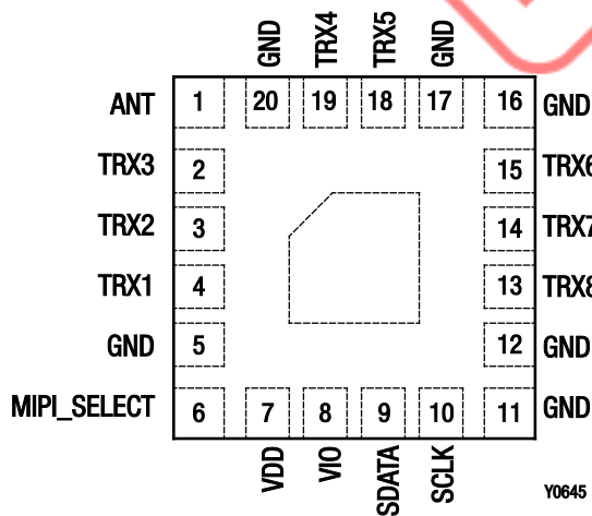
Figure 2. SKY13561-670LF Pinout – 20-Pin QFN (Top View)
