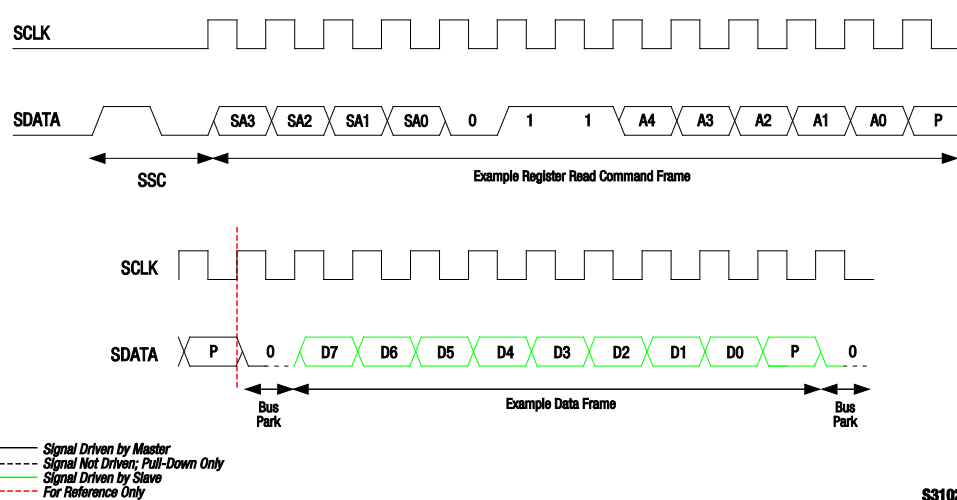
Figure 5. Register Read Command Timing Diagram
