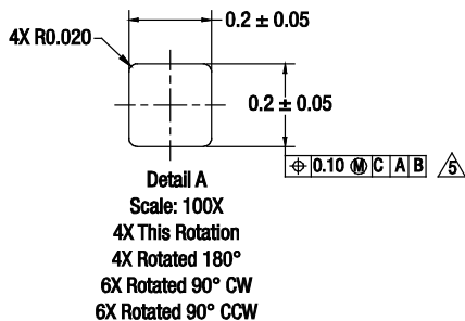
Figure 11. SKY13561-670LF 20-Pin QFN Package Dimensions
