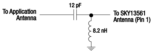
ESD Circuit 2
