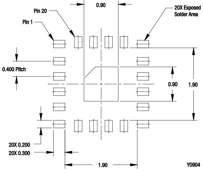
Figure 9. SKY13561-670LF PCB Layout Footprint (Top View)
