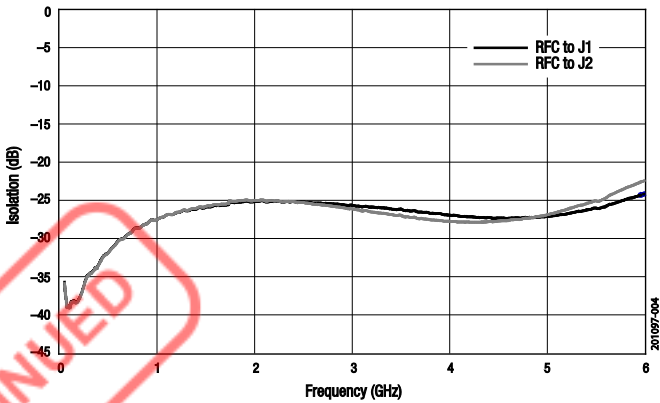
Figure 4. Typical Isolation
