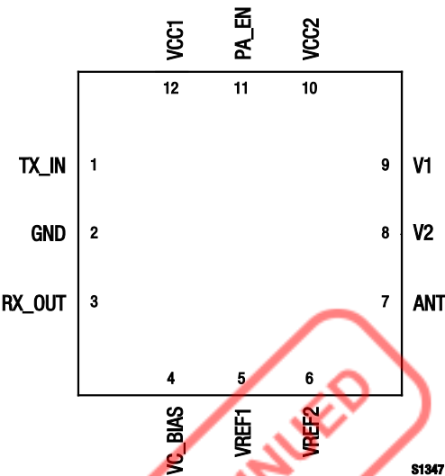
Figure 2. SKY65338-21 Pinout (Top View)
