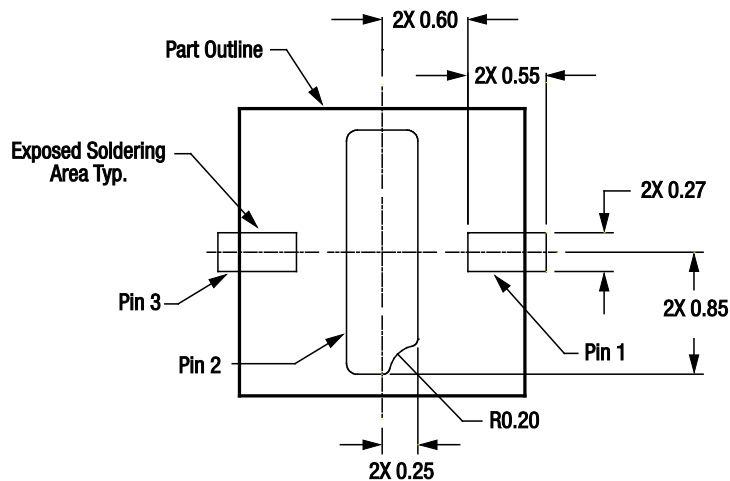
Figure 8. CLA4605-085LF PCB Layout Footprint
