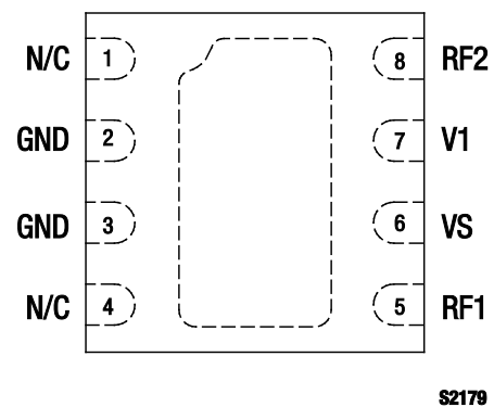
Figure 2. SKY13347-360LF Pinout (Top View)
