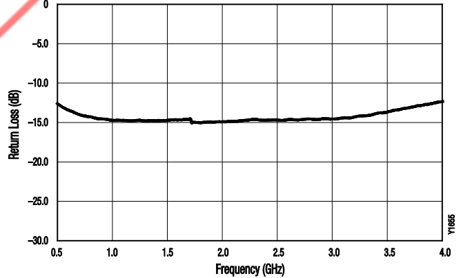
Figure 6. RF2 Return Loss (Isolation State) vs Frequency
