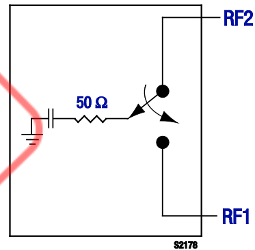
Figure 1. SKY13347-360LF Block Diagram
