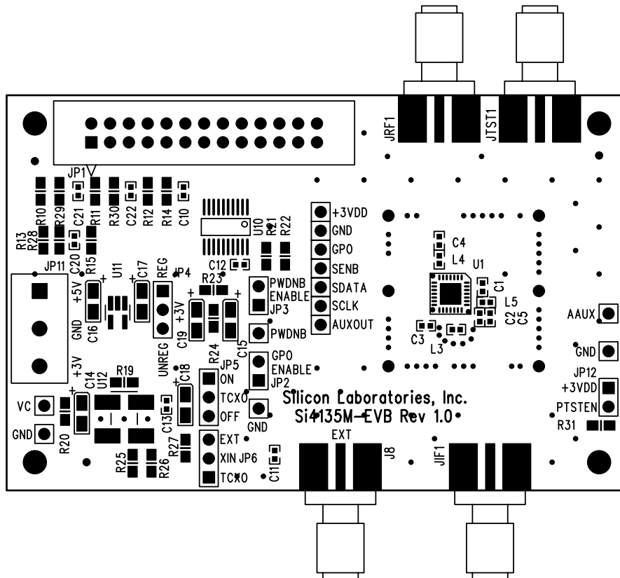
Figure 36. Si4135M Silkscreen
