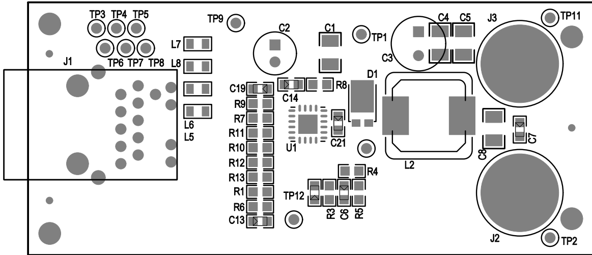
Figure 9.1. Top Silkscreen
