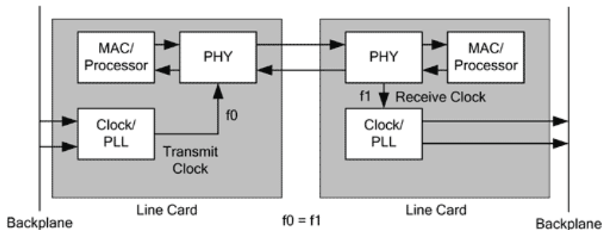
Figure 2. Example of Synchronous Clocking
