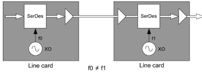
Figure 1. Example of Asynchronous Clocking
