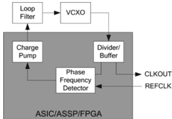
Figure 3. Partially Integrated PLL in ASIC
