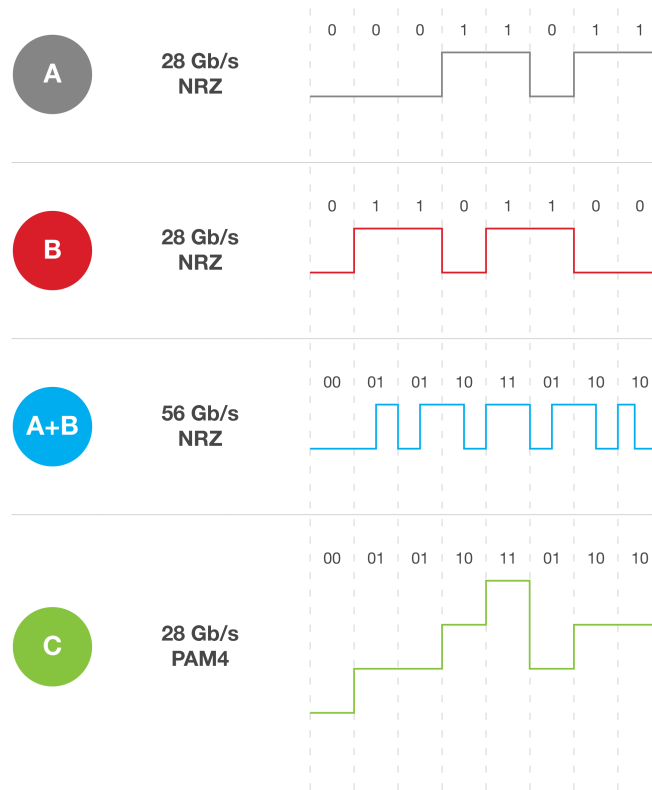
Figure 2.2. Signal Levels and Encoding of SNR vs. PAM-4
