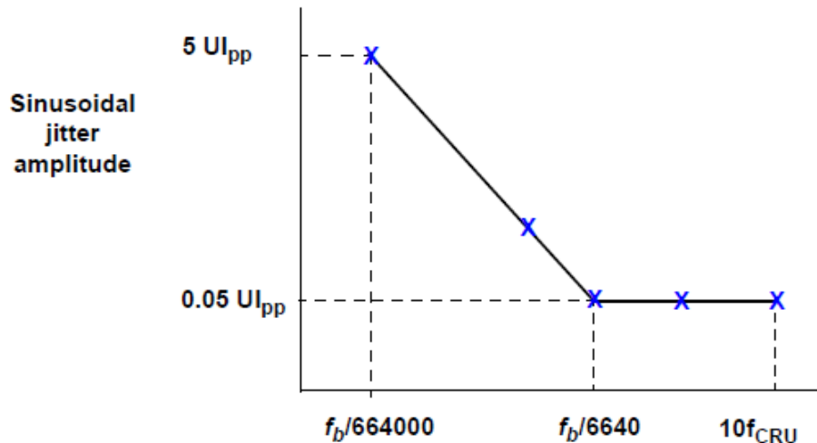
Figure 3.3. Receiver Jitter Tolerance from OIF-CEI-04.0 Standards 1
