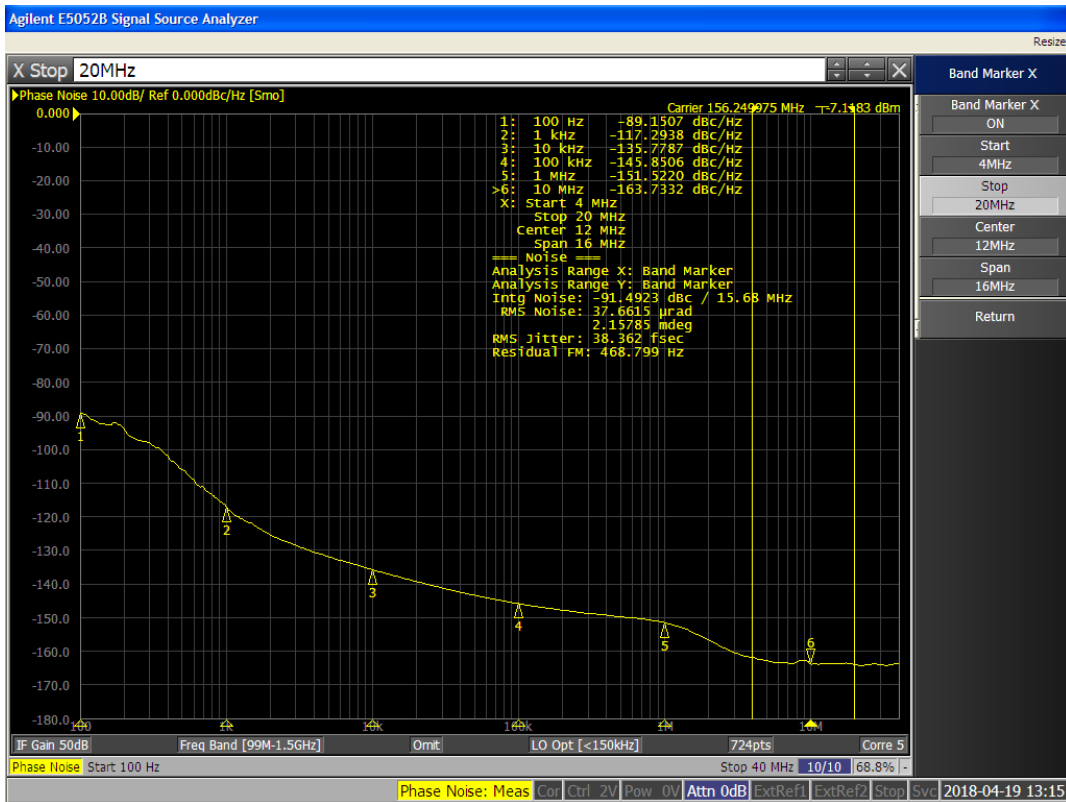
Figure 4.3. Phase Noise Plot Si5395P RMS Jitter 4 MHz–20 MHz Integration Band
