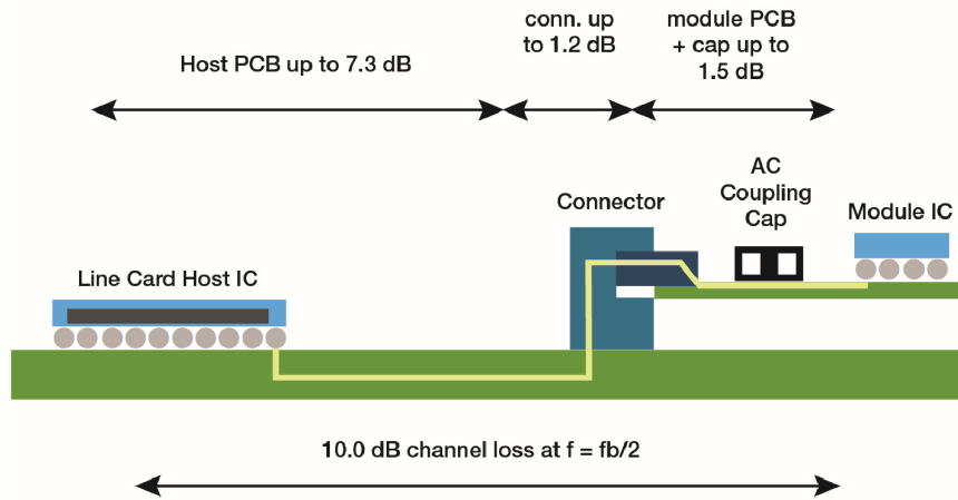
Figure 3.2. VEI-56G-VSR-PAM4 Channel Reference Model 1
