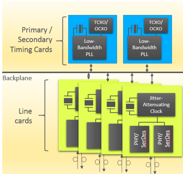
Figure 4.1. Line Card Showing Jitter Attenuator used for Signal Integrity of the 56G SerDes
