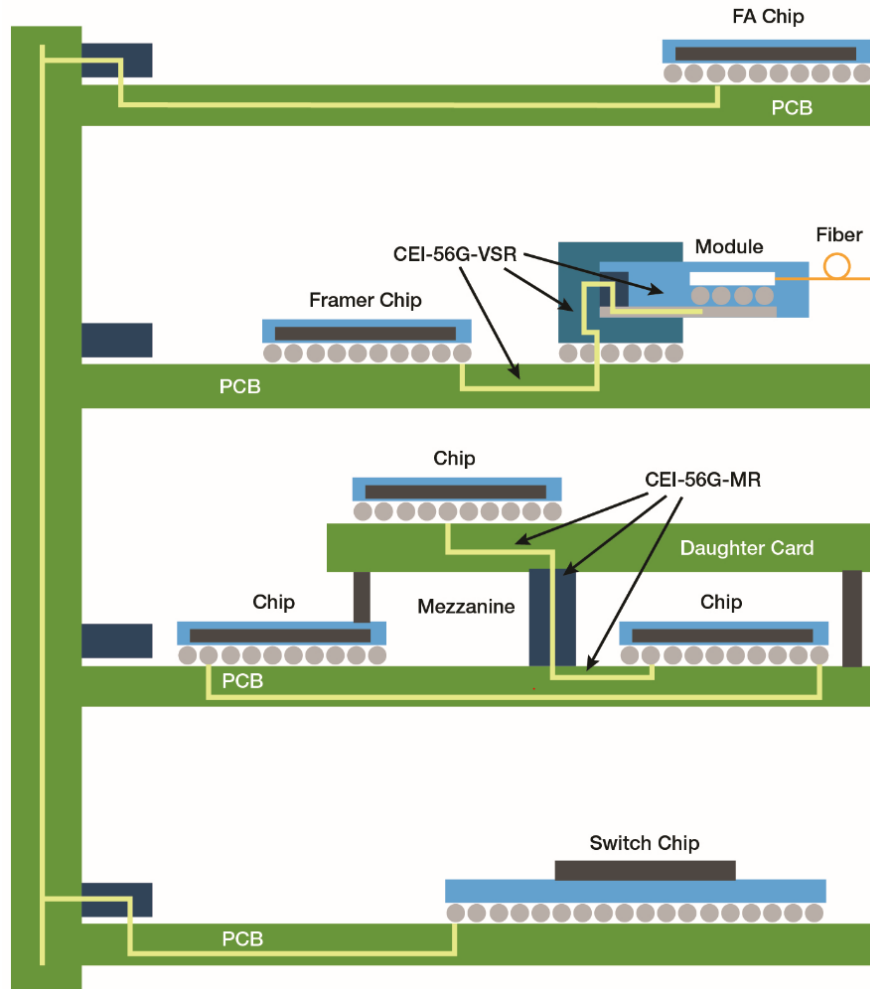
Figure 3.1. Different SerDes Interconnects of Varying Trace Lengths 1
