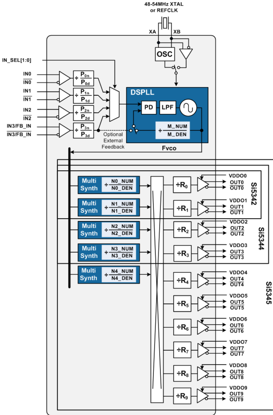
Figure 1.1. Functional Block Diagram
