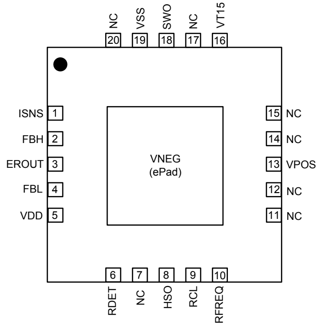
Figure 5.1. Si3404 Pinout
