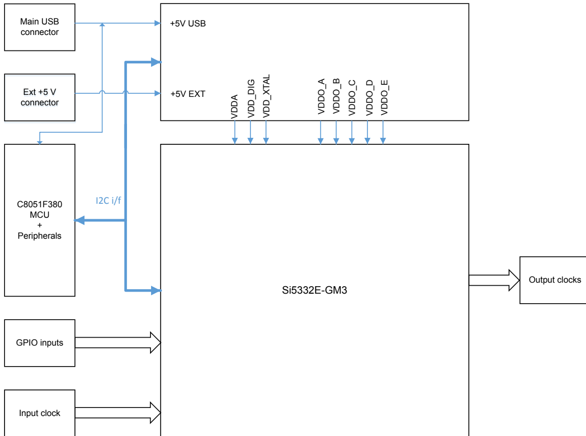
Figure 1.1. Si5332-12IX-EVB Functional Block Diagram
