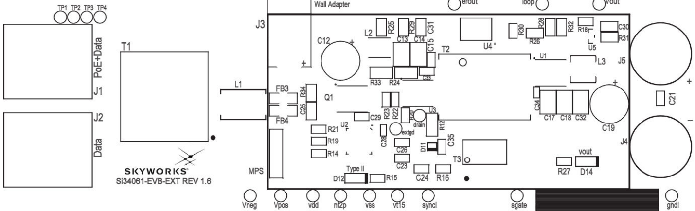
Figure 19.1. Primary Silkscreen
