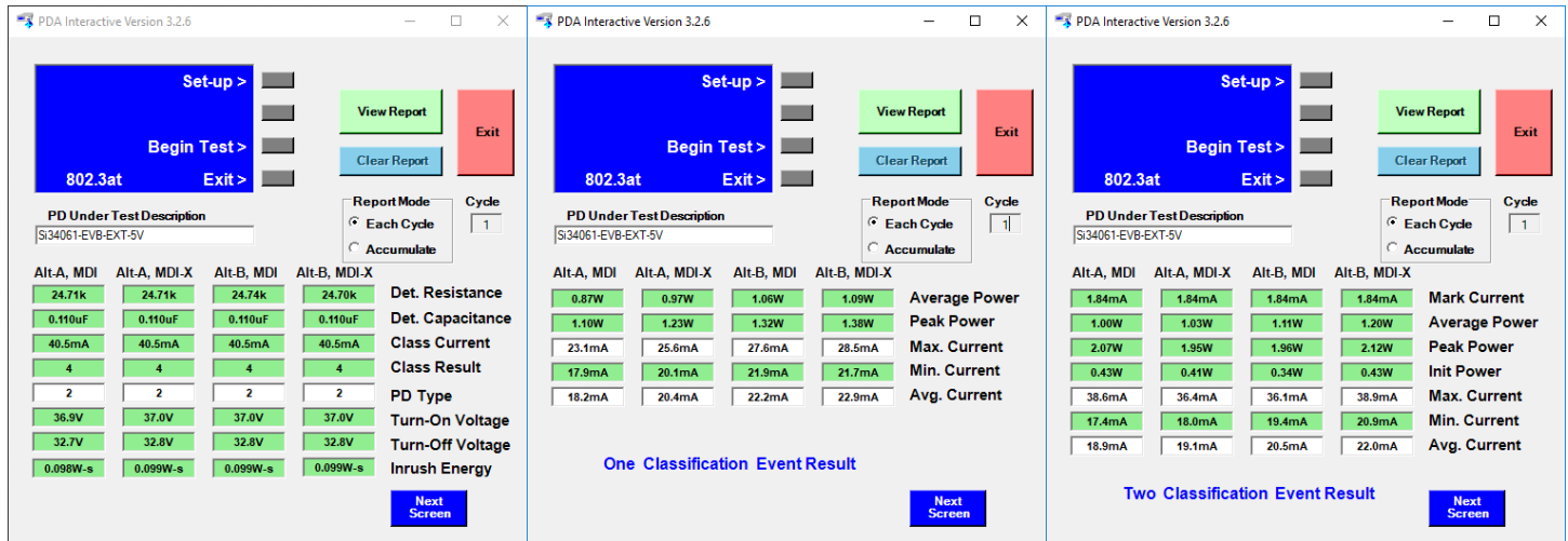
Figure 4.1. Si34061-EVB-EXT-5V PD SIFOS PoE Compatibility Test Results
