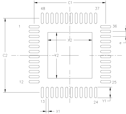
Figure 29. Si52208 Land Pattern
