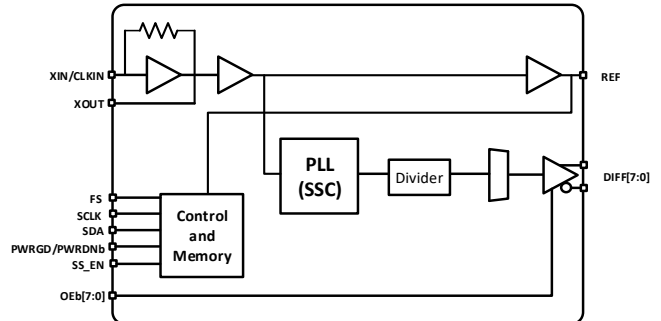
Figure 2. Si52208 Block Diagram 8-Output, 48-QFN
