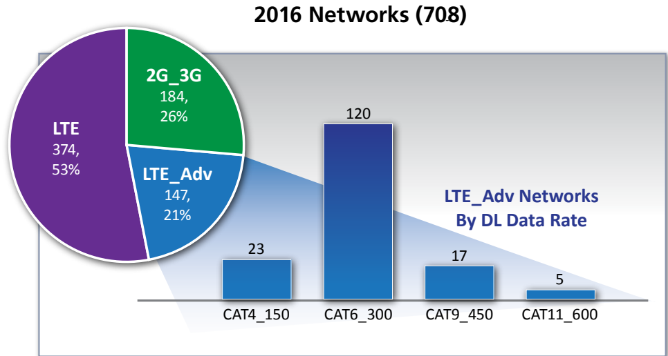
Figure 6. LTE Advanced (CA) Networks
