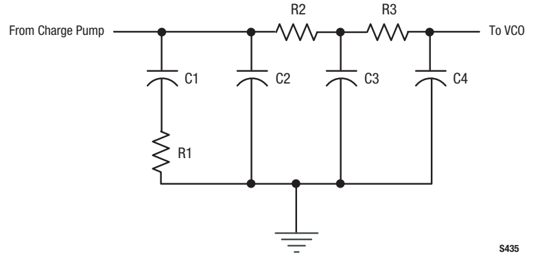
Figure 7. Loop Filter, More Reduction in Quantization Noise
