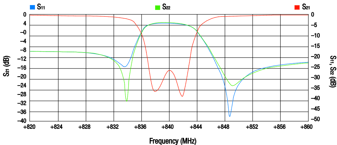
Figure 1: AMPS Band Reject Filter
