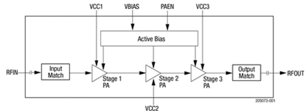
Figure 1. SKY66319-11 Block Diagram
